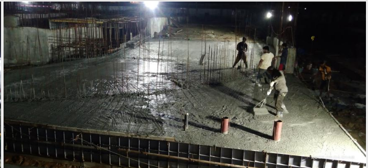
Ready mix concreting
